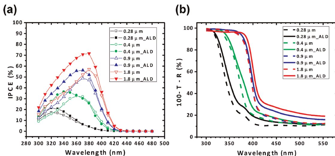
Figure 7. (a) IPCE (1.5 V vs RHE) for \text{TiO}_2 nanowires of different lengths is shown for nanowires with and without 150 ALD cycles. The EQE is mainly enhanced at \lambda = 320\text{--}380 nm. (b) 100 - \text{transmission} - \text{reflection} (%) for the corresponding \text{TiO}_2 nanowire arrays.
